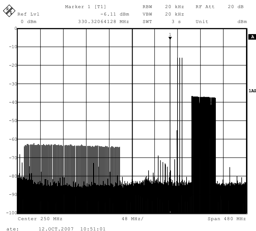
Figure 25. DAC5682Z Output Spectrum for Four Tone Groups
